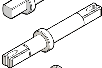
2.5 Motor Snap [x2] 228-3943-093
